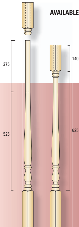
JB135 - Regent Pin Top Baluster Length: 1000mm Width: 42mm Pin Diameter: 25mm
