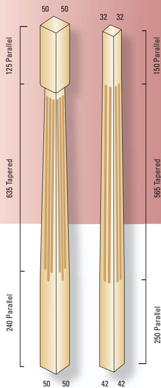
JB139 - Tudor Baluster Length: 1000mm Width: 50mm
